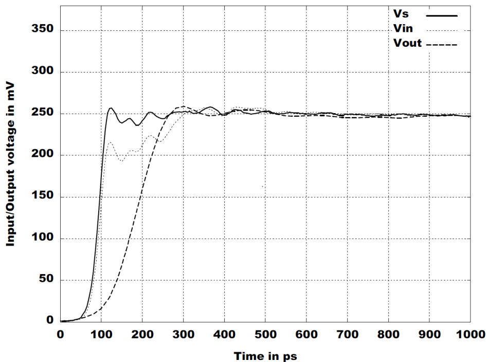
Fig. 4-10: Unloaded and loaded input signal and step response (for RT-ZS30)
